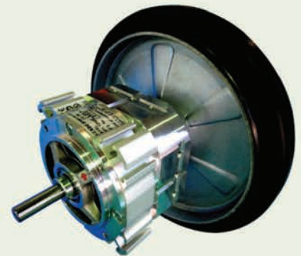
Bearing unit
